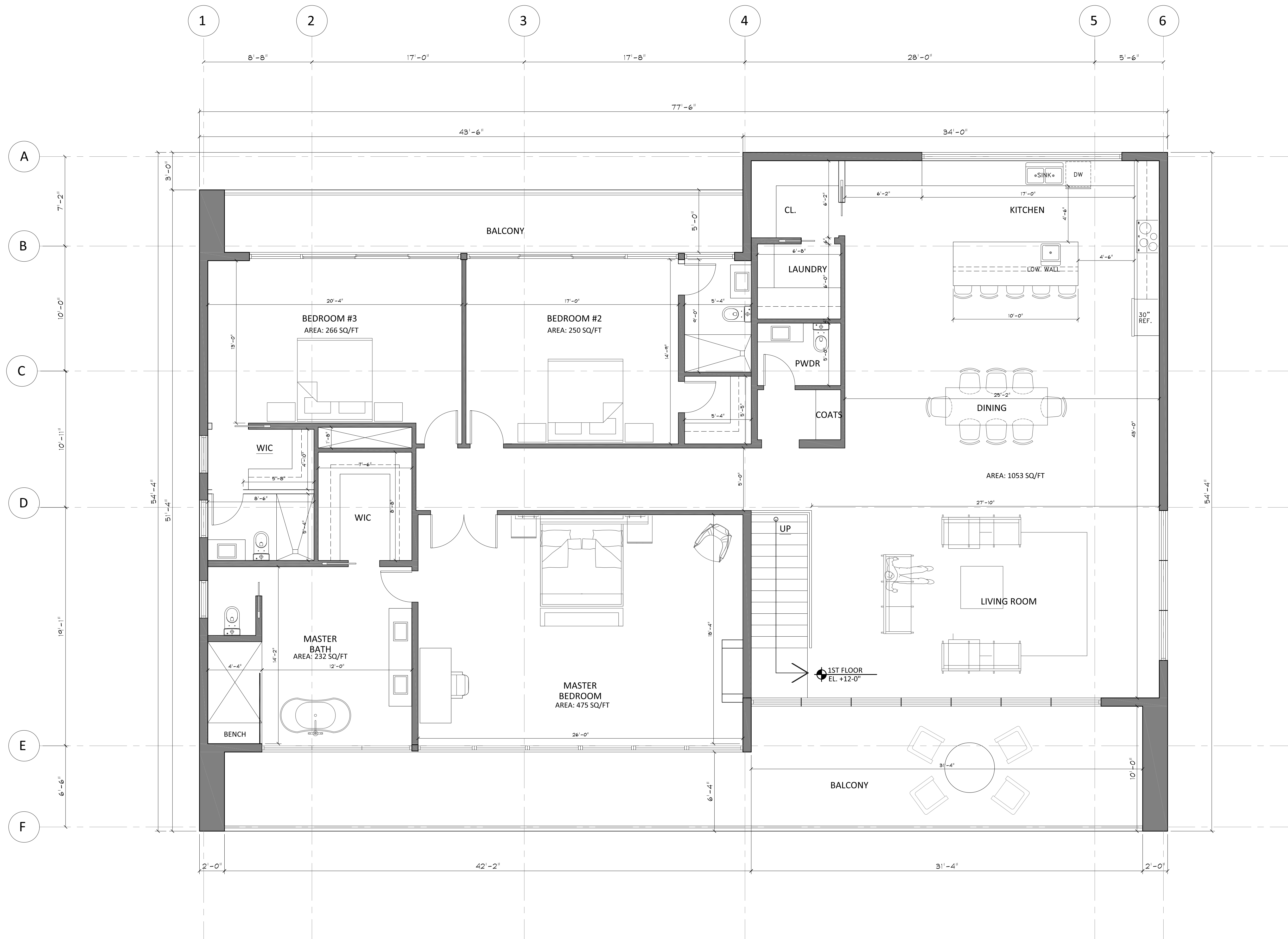
1ST FLOOR PLAN ESC: 1/4"=1'-0"
