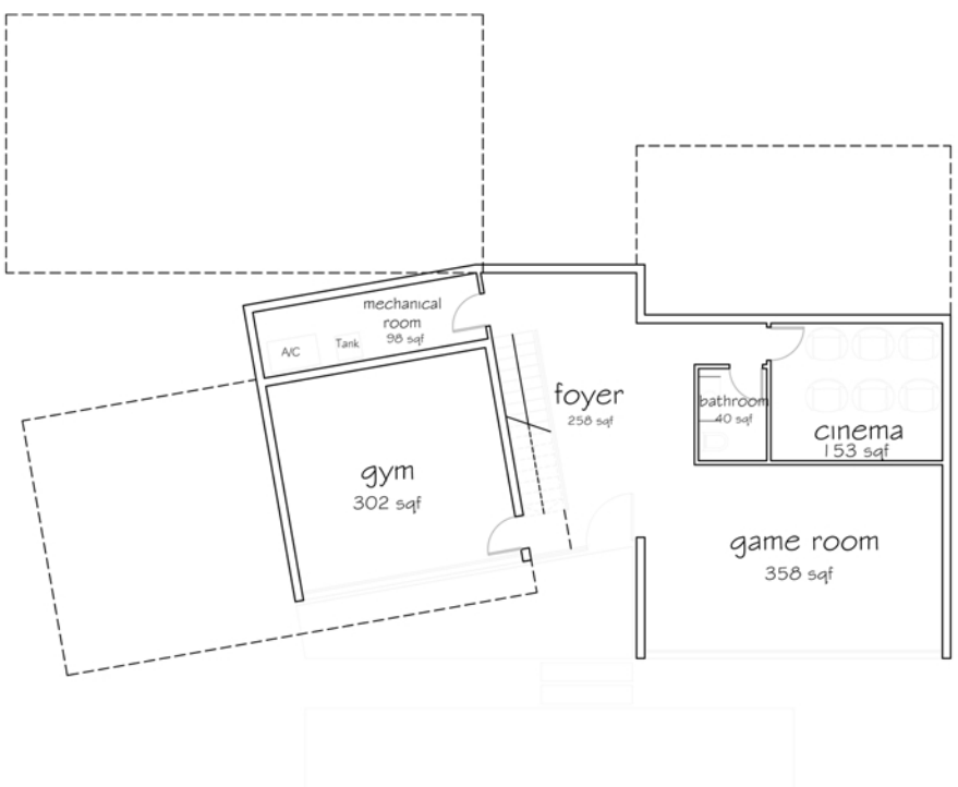
underground floor 1400sqf
